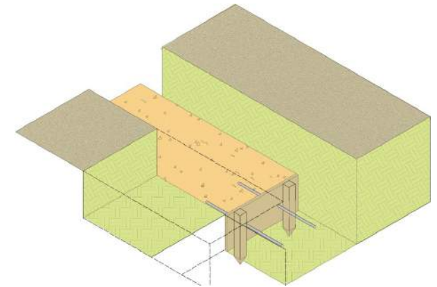
Figure 16: Using reinforcement bars across a joint
