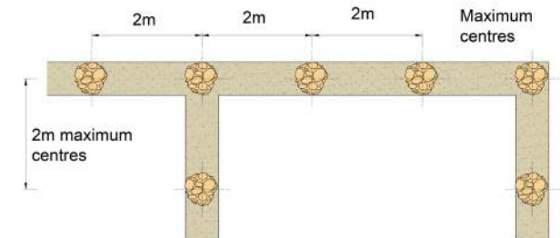
Figure 4: The intersection of adjacent reinforced concrete strips
