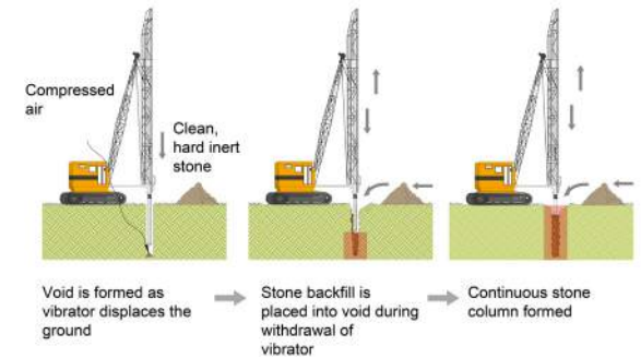
Figure 1: Vibratory techniques - dry bottom feed method
