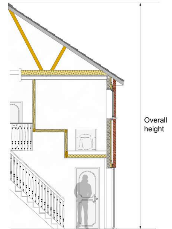
Figure 3: Overall height
