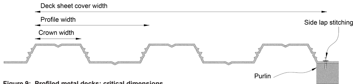
Figure 9: Profiled metal decks: critical dimensions
