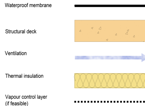
Figure 3: Cold roof (section)
