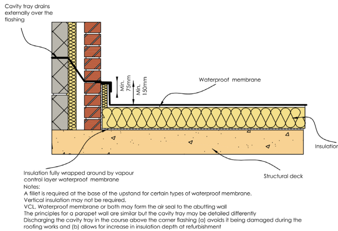
Figure 5: Principles of detailing: an example of warm deck roof at an abutment
