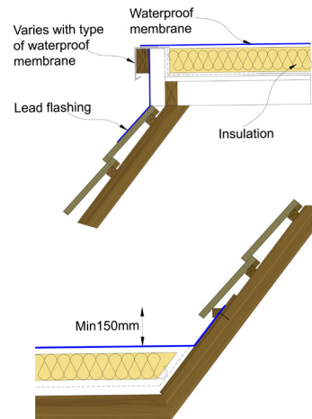
Figure 7: Detail: principles: flat roof interface to pitched roof
