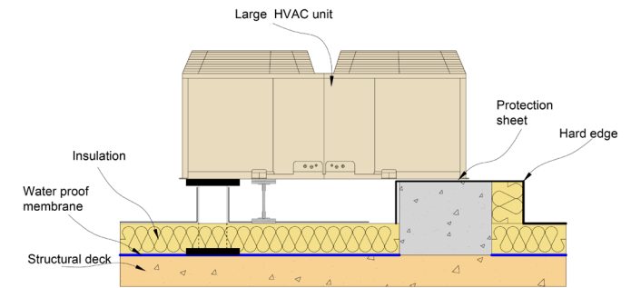
Figure 8: Detail – principles – plant support
