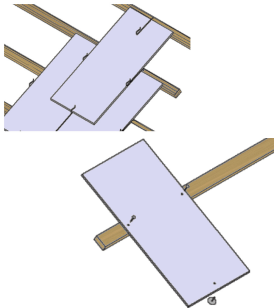
Figure 13: Fixing slates
