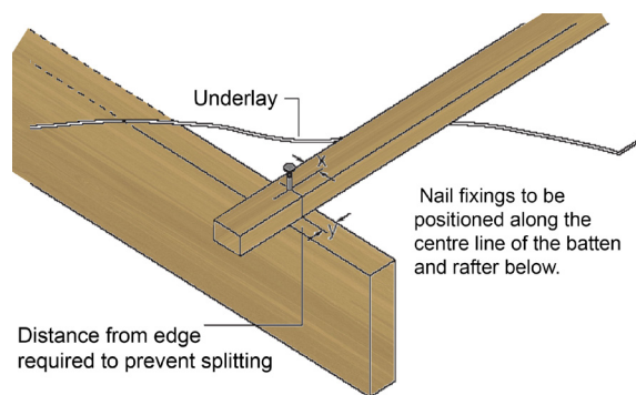
Figure 14: Fixing battens to rafters
