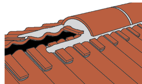
Figure 17: Ridge detail
