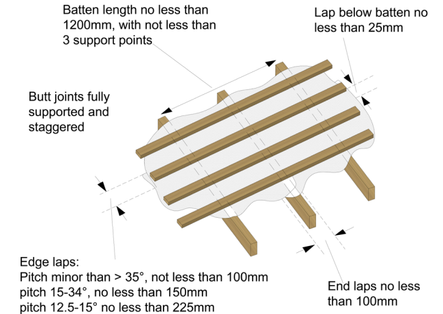
Figure 10: Roof underlay provision
