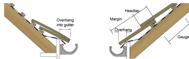
Figure 15: Eaves and bottom edge details
