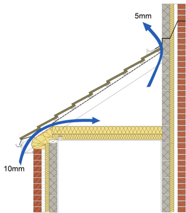
Figure 1: Mono-pitch/lean-to roof
