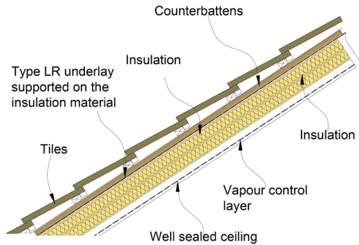
Figure 9: Warm roof construction (vapour breathable underlay)
