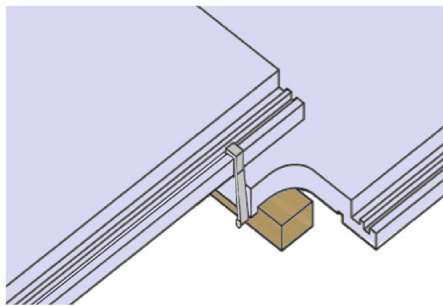
Figure 12: Tile clips
